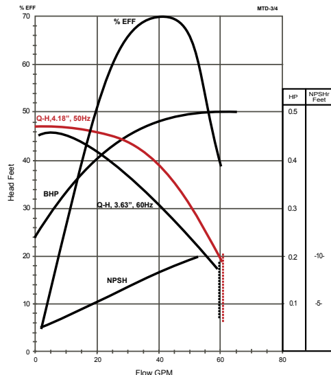
MTD3/4 THREADED HOUSING POLYPROP. PUMP WT. 10.5 LBS (4.8KG) MOTOR WT. 28 LBS (12.7KG)
