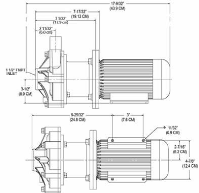
MTD3/4 THREADED HOUSING POLYPROP. PUMP WT. 10.5 LBS (4.8KG) MOTOR WT. 28 LBS (12.7KG)
