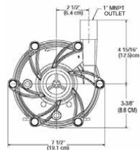
MTD3/4 THREADED HOUSING POLYPROP. PUMP WT. 10.5 LBS (4.8KG) MOTOR WT. 28 LBS (12.7KG)
